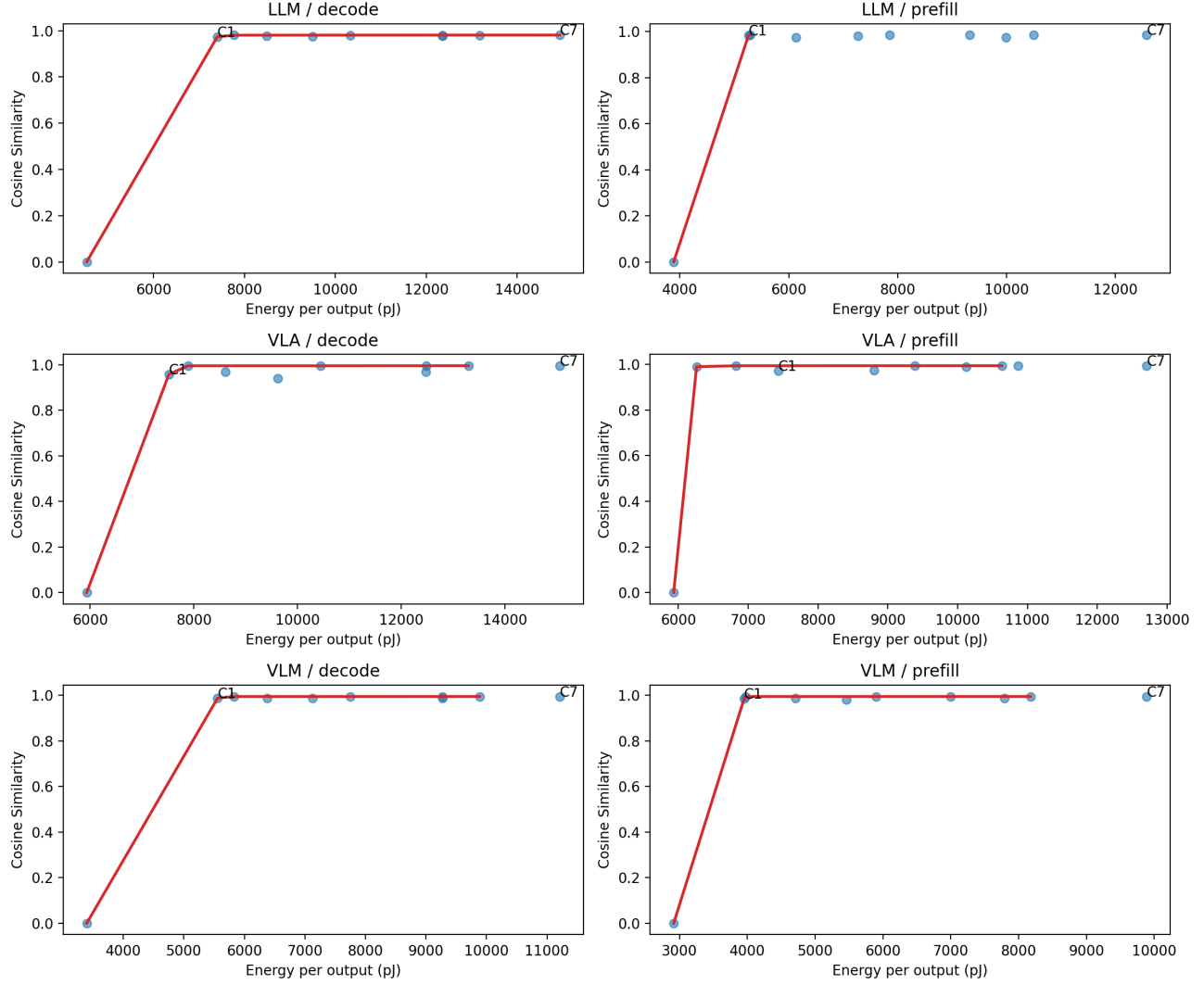
Fig. 4. Accuracy–energy Pareto panels for the completed 3-workload \times 2-phase sweep. C7 (NVFP4-like) is consistently high energy, while C1 (MXFP4-like) often lies near the low-energy knee.
