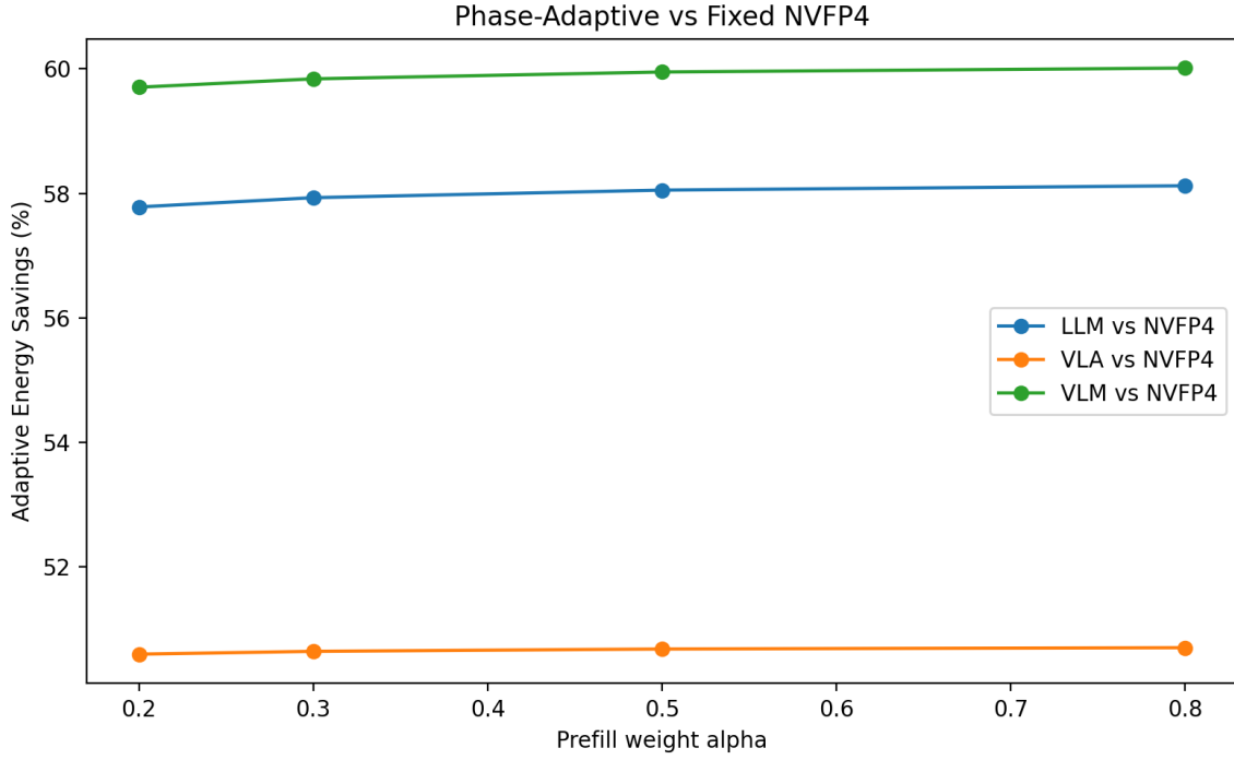
Fig. 5. Phase-adaptive energy savings versus fixed NVFP4-like C7 as the prefill weighting \alpha changes.
