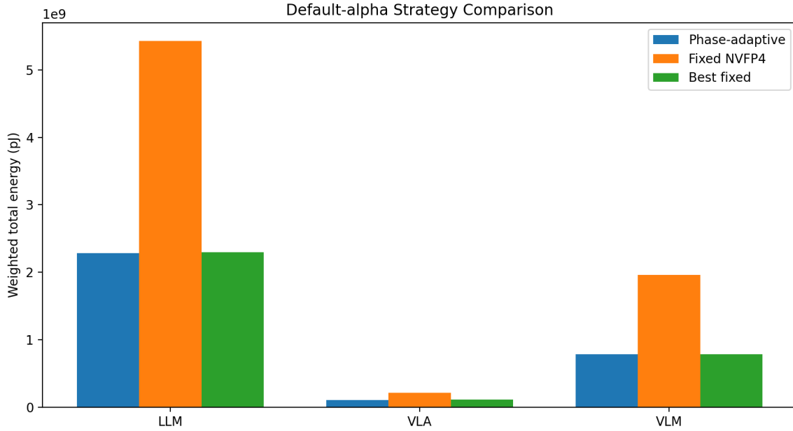
Fig. 6. Weighted-energy comparison at the default workload-specific \alpha values. Phase-adaptive equals best-fixed for VLM because both phases select C1.
