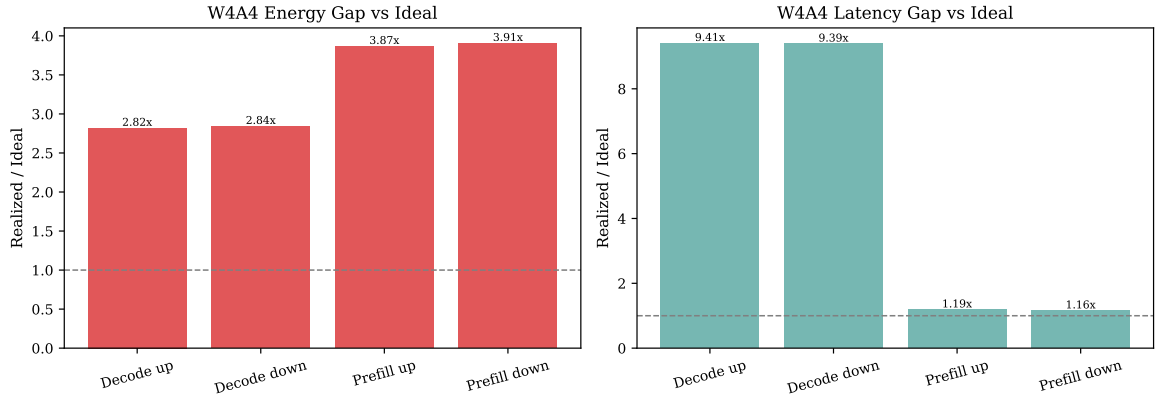
Fig. 3. Realized NVFP4 cost relative to ideal (zero-overhead) W4A4. The 2.8–3.9 \times energy gap is the optimization headroom targeted by our rescale pipeline DSE.
